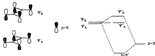
Figure 3. Perturbative interaction of filled heteroatomic p-\pi -orbital with the NBMOs of tetramethylethane. 9
