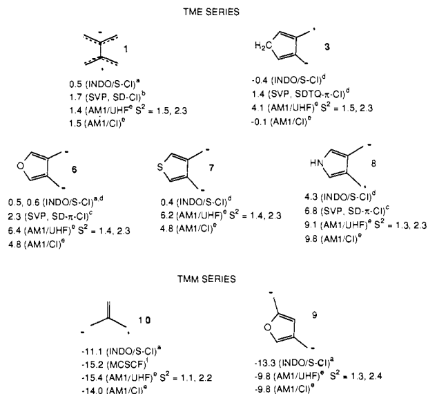
Figure 2. Calculated energy separations ( E_T - E_S , kcal/mol) of lowest singlet and triplet states of biradicals. a Reference 6. b Reference 8. c Reference 9. d Reference 7. e This work. f Reference 15.
